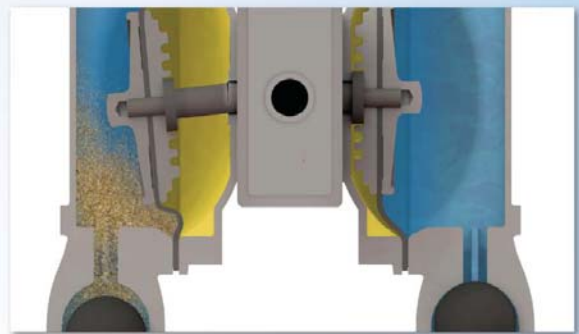
Setting solids collect inside pump, causing damage & affecting operation
